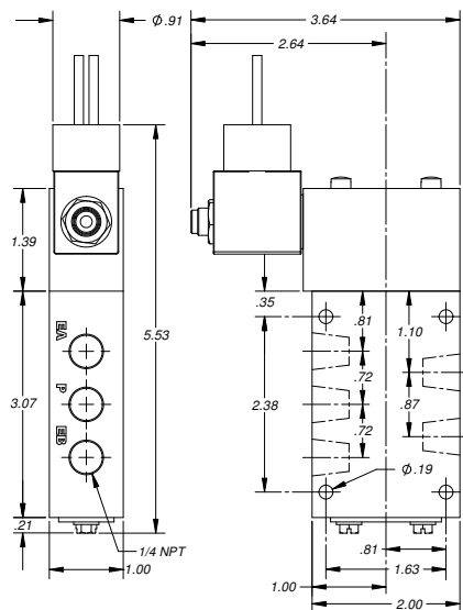
Single Solenoid M3951701-X
