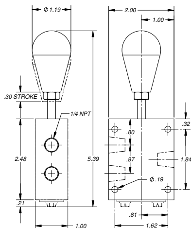
3-Way M3820701 or M3820702
