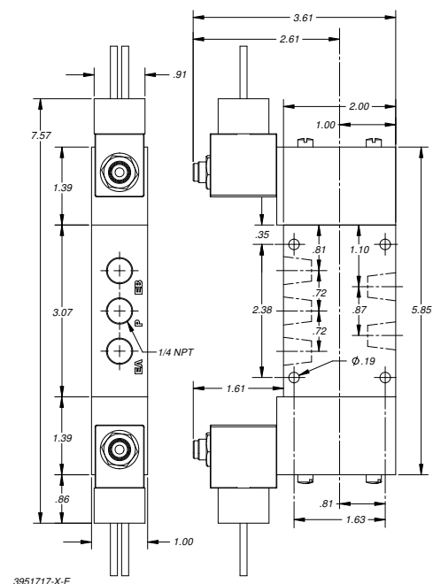
Double Solenoid M3951717-X-E
