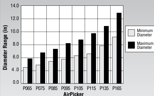
Large AirPicker Size Ranges
