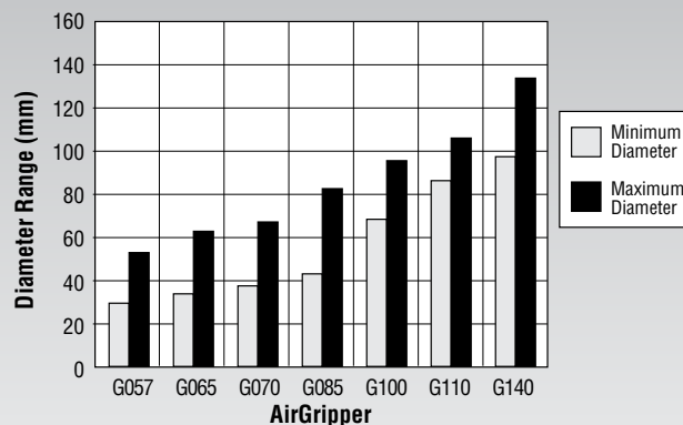
Large AirGripper Size Ranges
