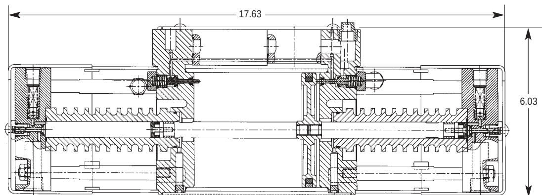
Double-ended Booster
