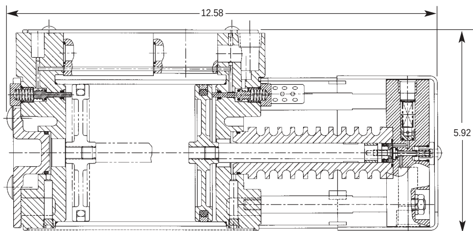
Single-ended Booster
