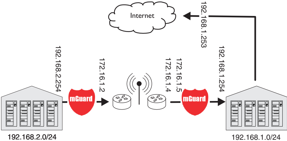
Figure 2-5 WLAN via VPN
