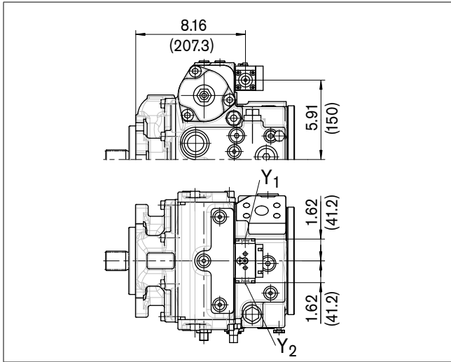
HT Hydraulic control, direct controlled
